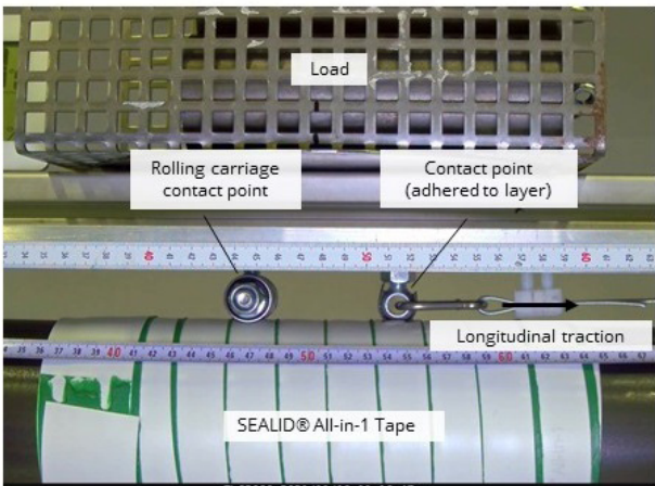
Test setup – Detailed view
